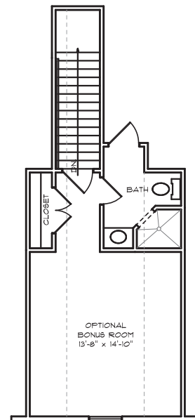
OPTIONAL SECOND FLOOR PLAN (adds 338 Heated Sq. Ft.)
