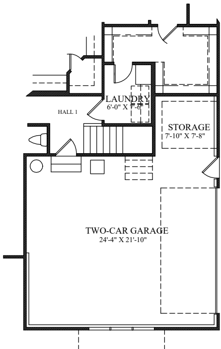
First Floor/Garage
