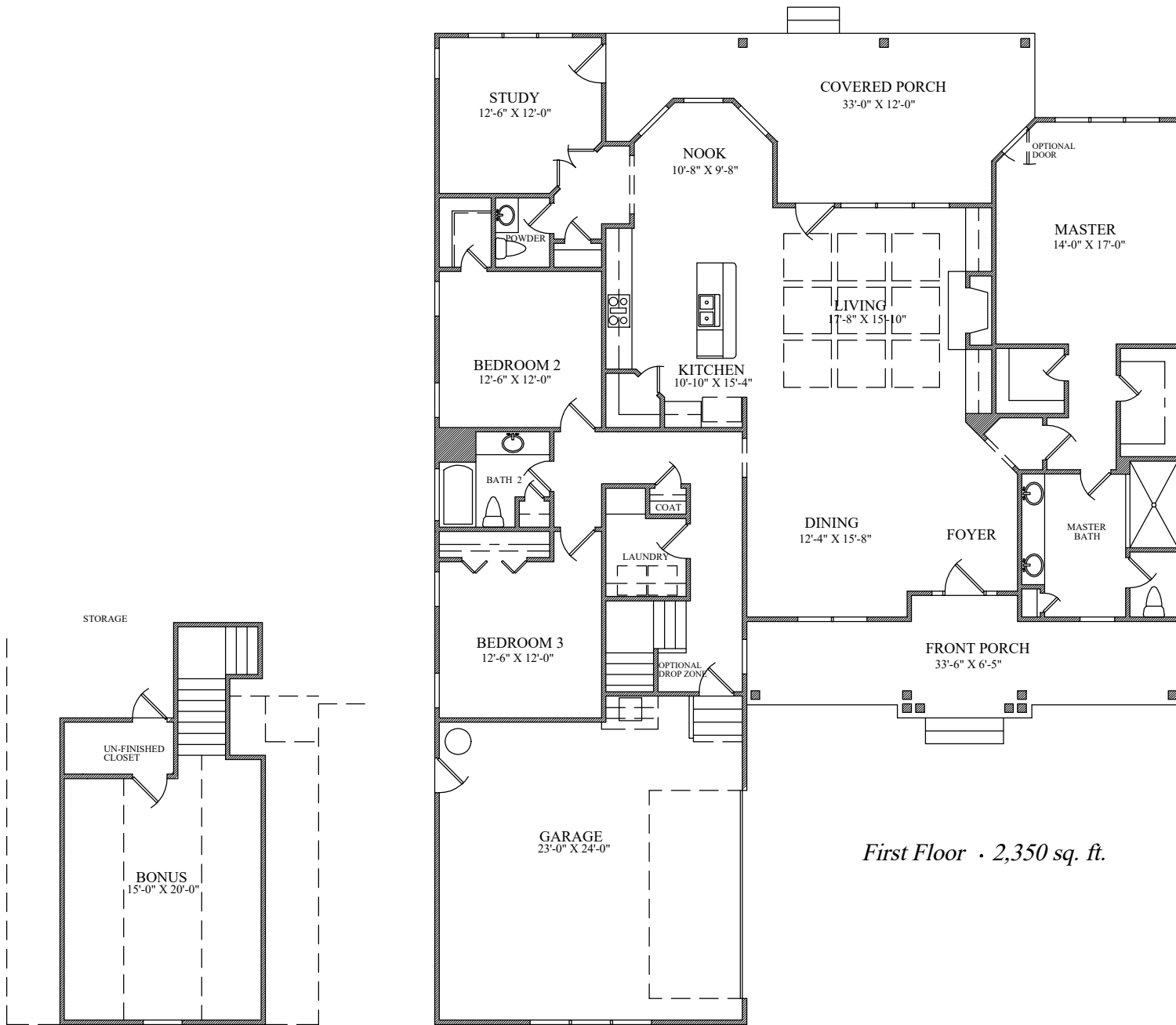
Bonus Floor . 314 sq. ft.
