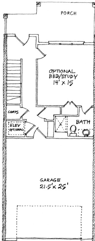
UNIT B GROUND FLOOR PLAN OPTION 2
