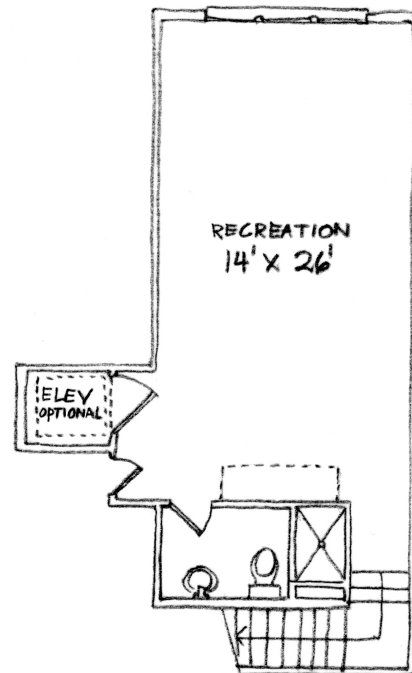
UNIT B OPTIONAL THIRD FLOOR
