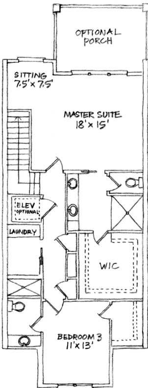
UNIT B SECOND FLOOR PLAN OPTION 2
