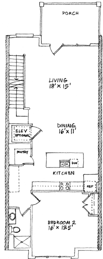
UNIT B FIRST FLOOR PLAN
