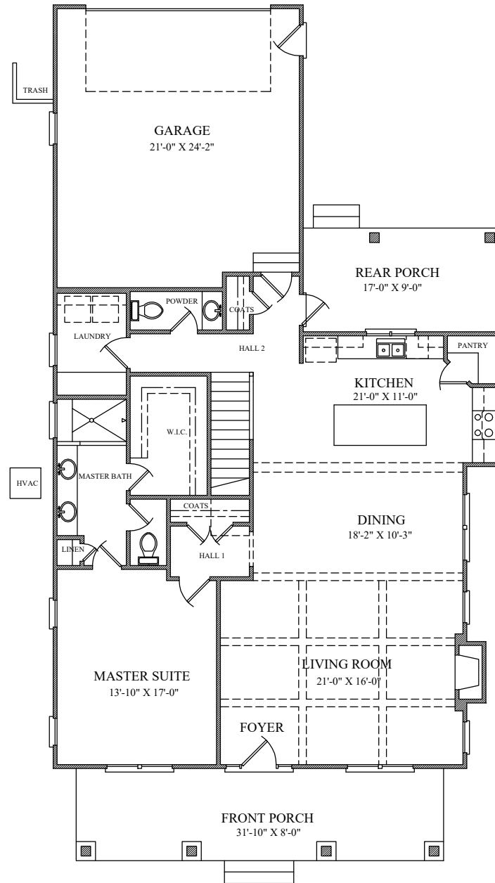
1,490 sq. ft. · First Floor
