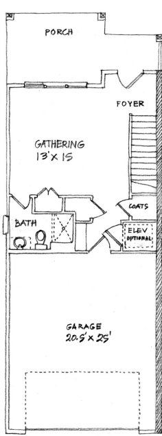
UNIT A GROUND FLOOR PLAN OPTION 1
