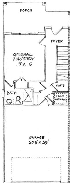
UNIT A GROUND FLOOR PLAN OPTION 2
