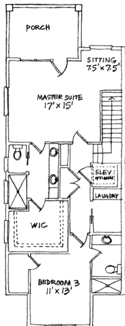
UNIT A SECOND FLOOR PLAN
