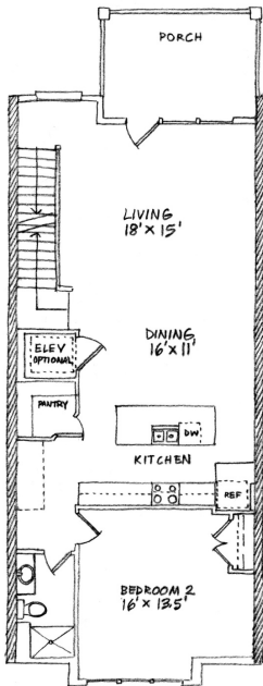
UNIT B FIRST FLOOR PLAN
