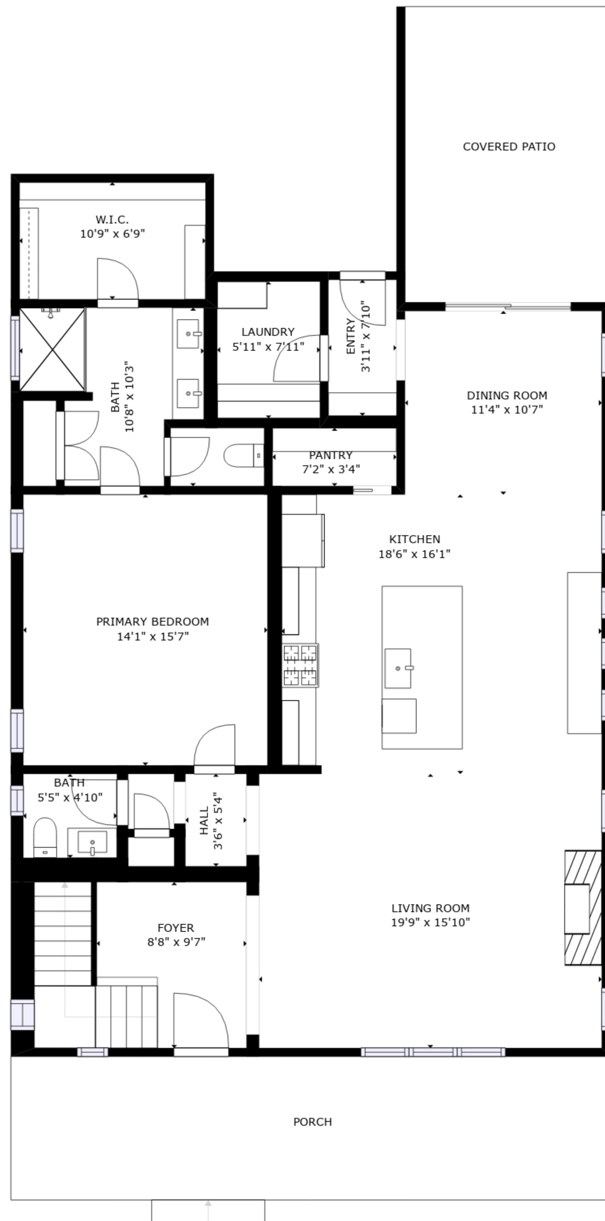
FLOOR 1
