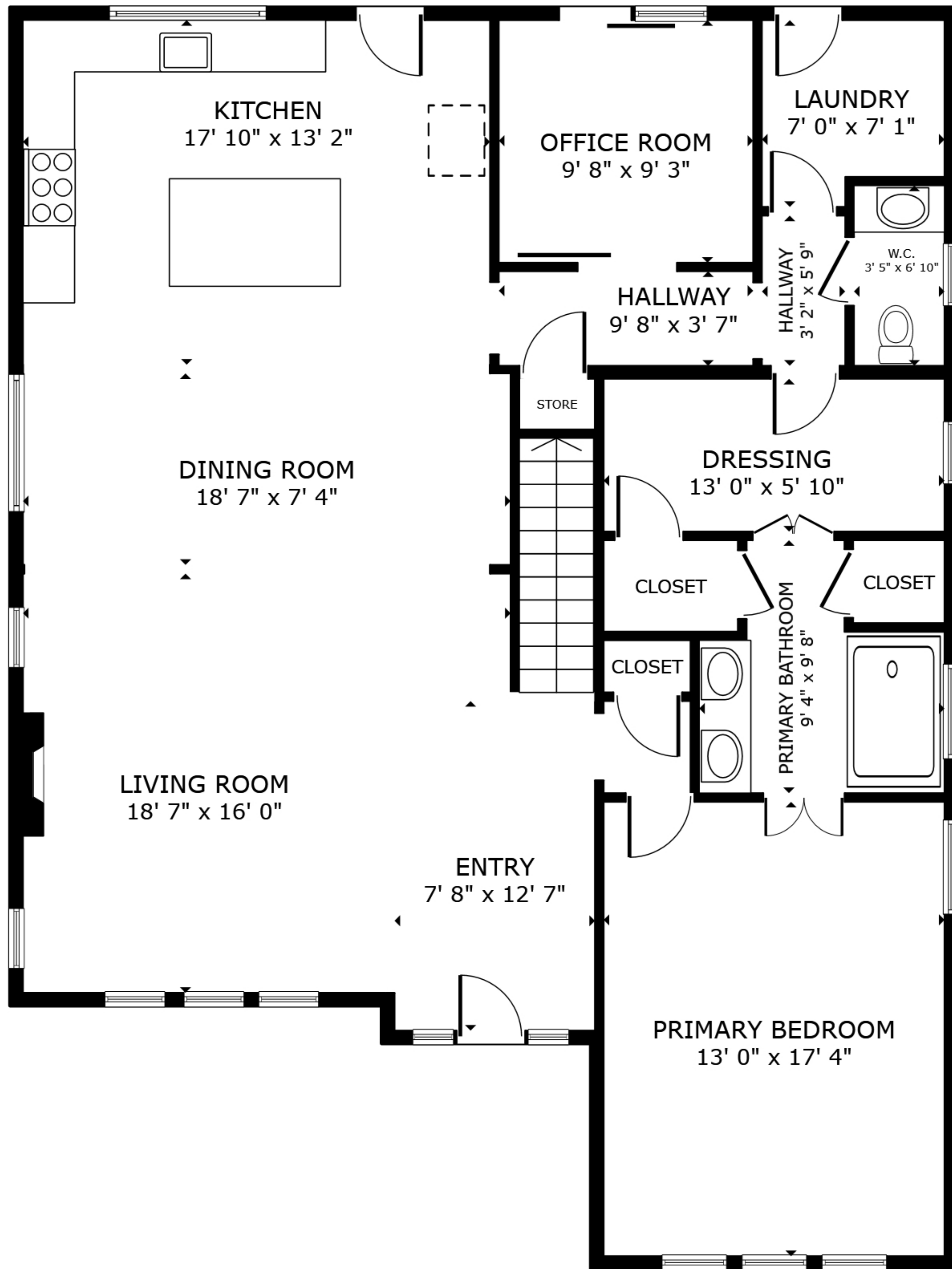
FLOOR 1
